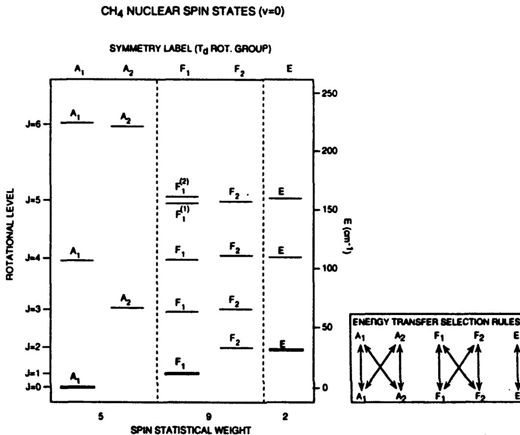
Fig. 2. Relevant nuclear spin symmetries (A,E, F) and collisional pathways for the CH 4 rotational manifold.
